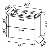
OUE 80 II/2 WH OUE 80 II/2 GRAY/ANT OUE 80 II/2 GRAY/OAK
