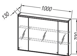
TO 100 BL - LED, SW, S
