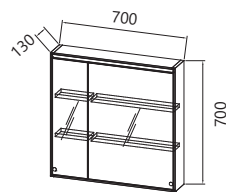
TO 70 BL - LED, SW, S
